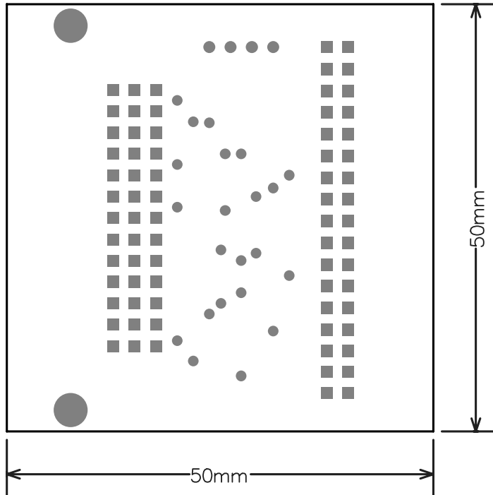
Mechanical Layer 1
